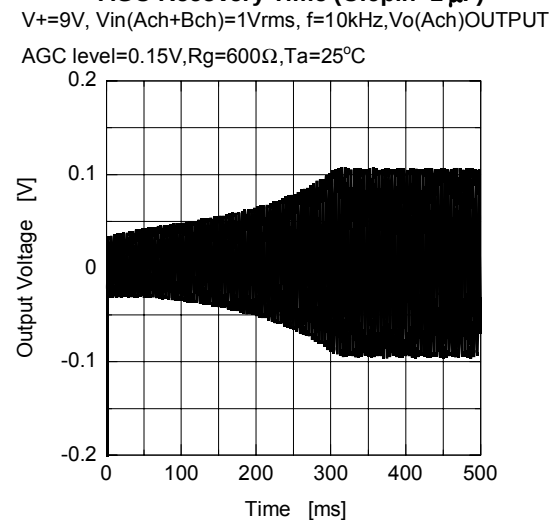
AGC Recovery Time (C:9pin=1μF)
