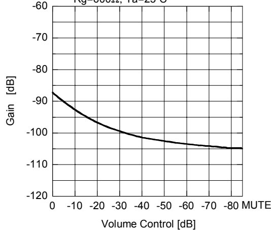
Output Noise vs Volume Control
