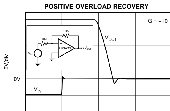
Time (0.5 \mu\text{s}/\text{div} ) Figure 38.
