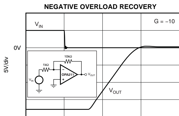
Time (0.5 \mu\text{s}/\text{div} ) Figure 37.
