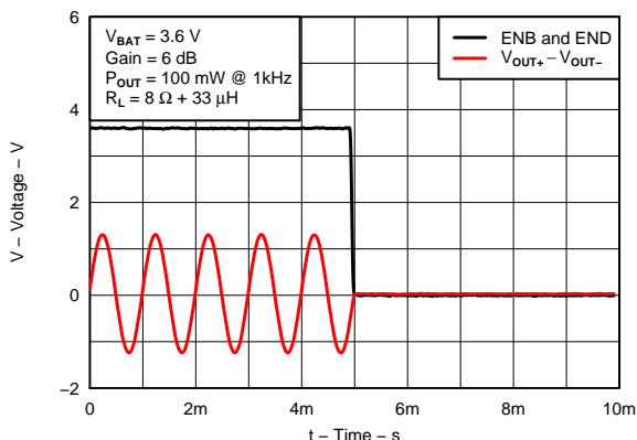
Figure 16. SHUTDOWN TIMING
