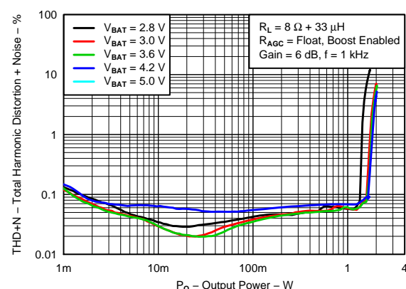
Figure 6. TOTAL HARMONIC DISTORTION + NOISE vs OUTPUT POWER
