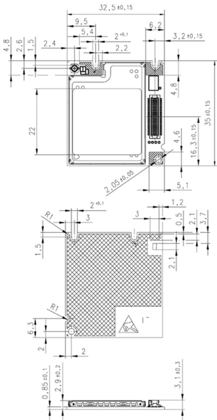
Figure 35: Mechanical dimensions of MC37i (all dimensions in millimeters)
