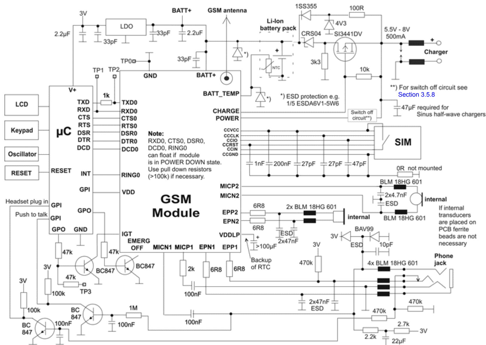
Figure 40: Schematic diagram of MC37i sample application
