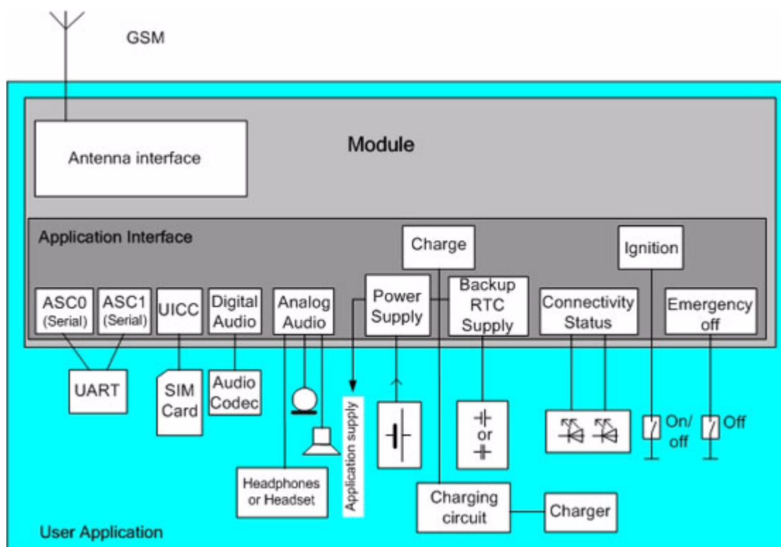
Figure 1: MC37i system overview
