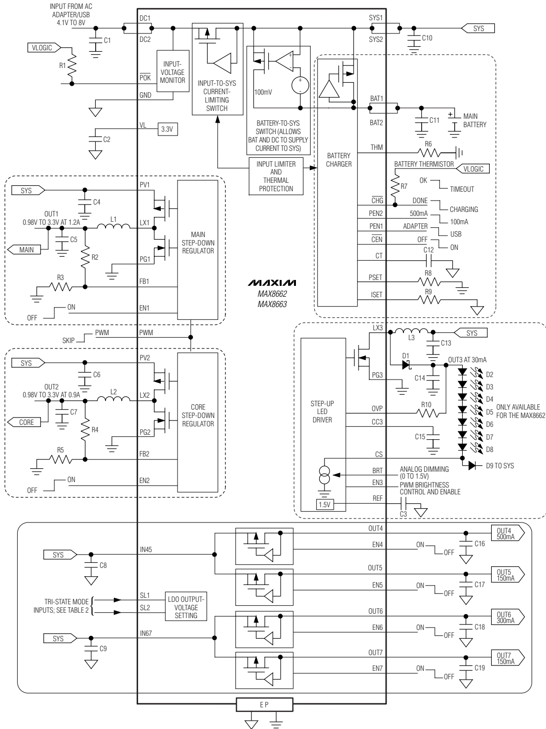
Figure 1. Block Diagram and Application Circuit
