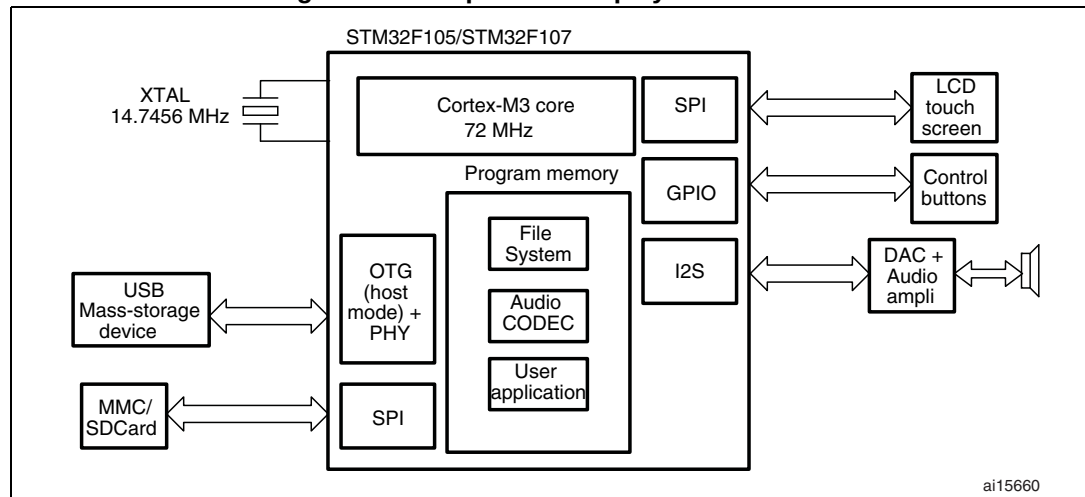
Figure 53. Complete audio player solution 1
