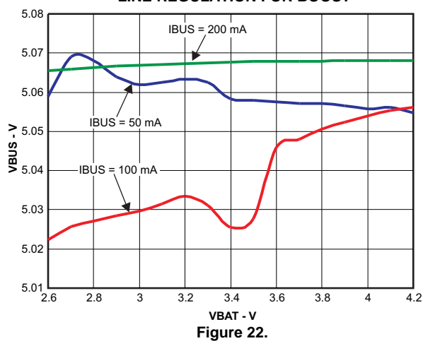
LINE REGULATION FOR BOOST
