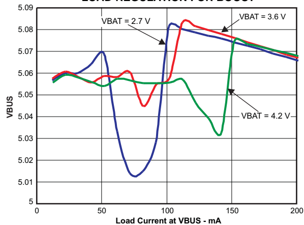
LOAD REGULATION FOR BOOST
