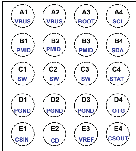
bq24153A/8 (Top View)
