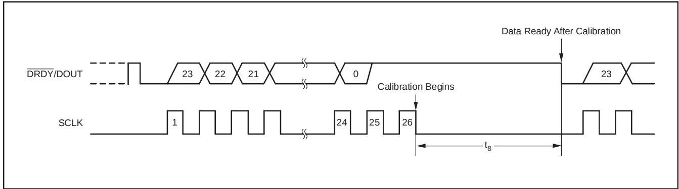
Figure 36. Offset-Calibration Timing
