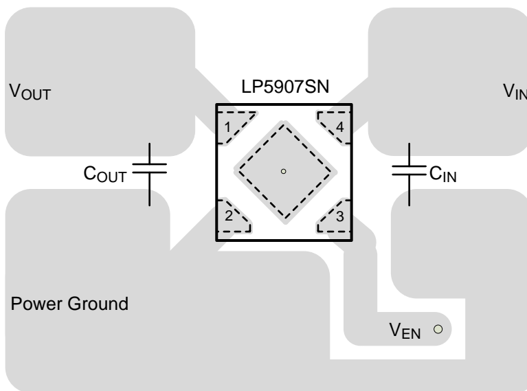
Figure 24. LP5907SN-xx (X2SON) Typical Layout
