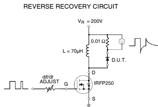
Fig. C.T.5 - Reverse Recovery Parameter Test Circuit
