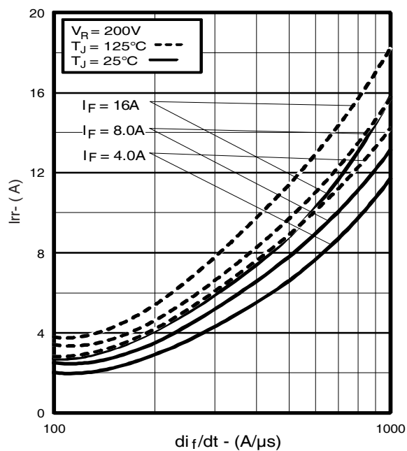
Fig. 20 - Typical Recovery Current vs. di_f/dt
