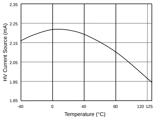
Fig. 5 HV Current source(Vcc=9V) vs. Temperature
