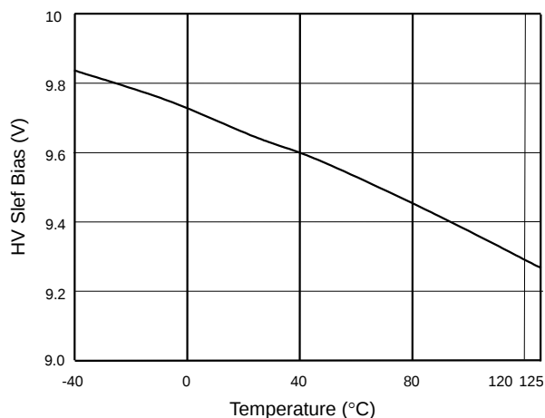
Fig. 3 HV Slef Bias vs. Temperature
