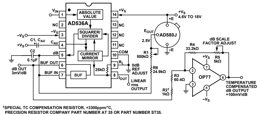
Figure 7. dB Connection
