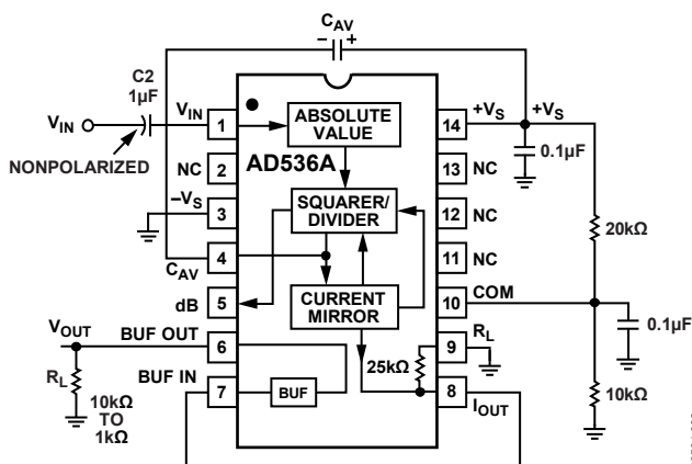
Figure 17. Single-Supply Connection
