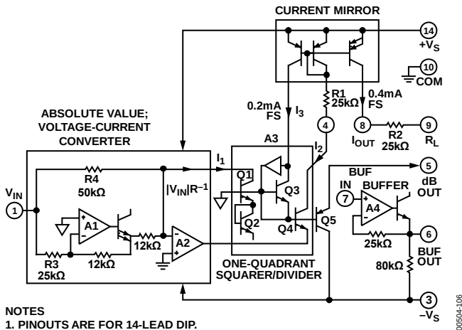
Figure 6. Simplified Schematic
