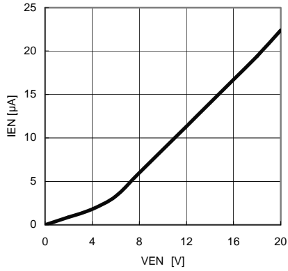
Fig.16 VEN-IEN
