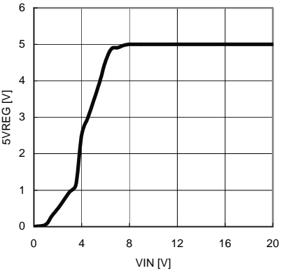
Fig.15 VIN-5VREG
