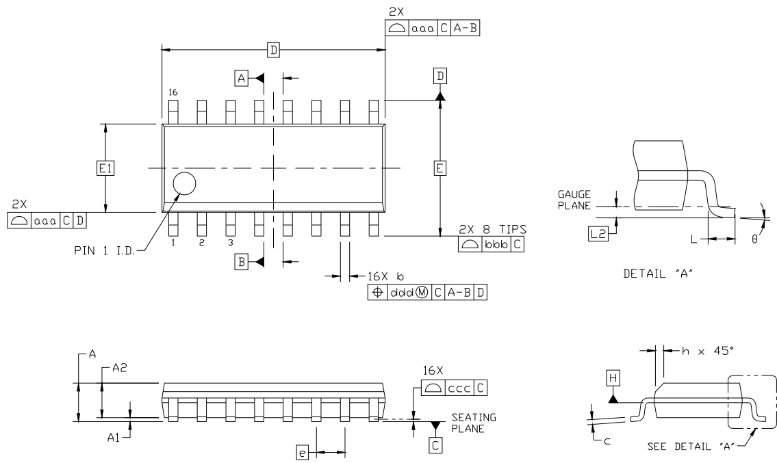
Figure 3. 16-Pin SOIC
