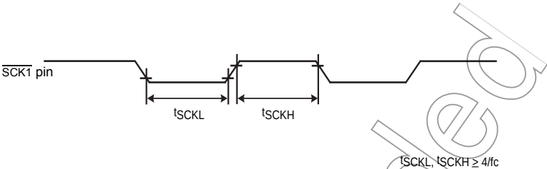
Figure 14-3 External Clock
