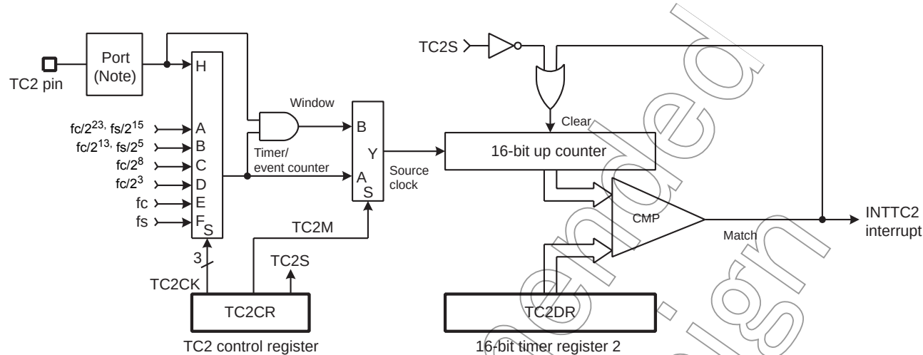
Figure 9-1 Timer/Counter2 (TC2)
