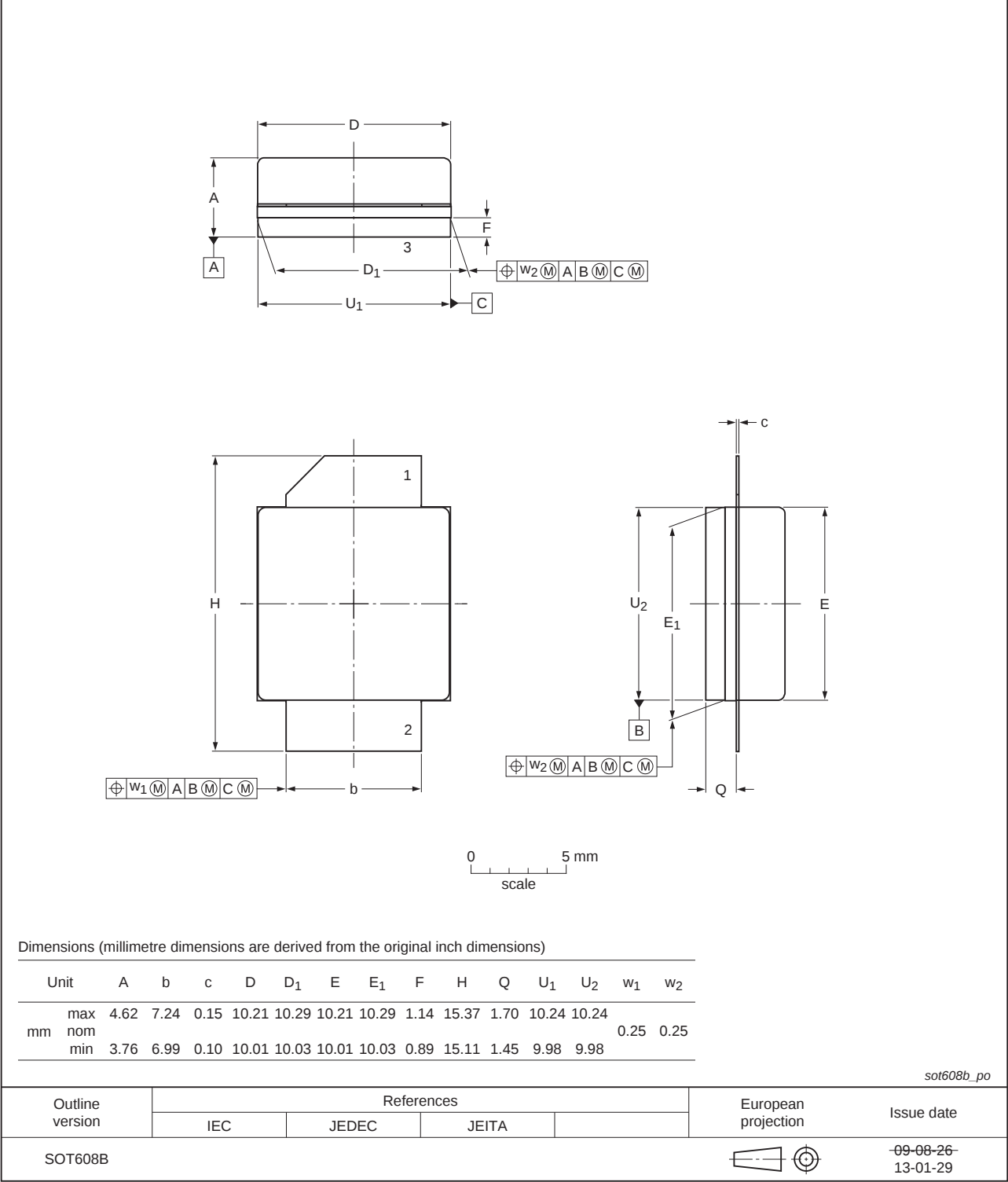
Ceramic earless flanged package; 2 leads SOT608B
