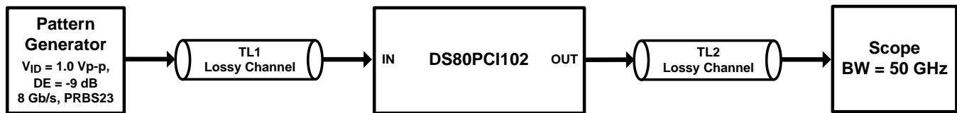
Figure 11. Test Setup Connections Diagram
