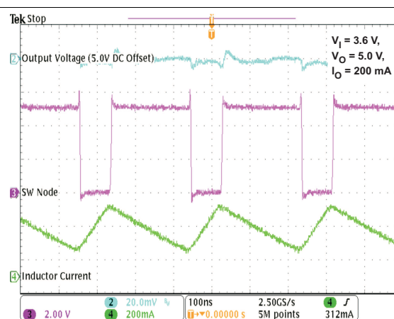
Figure 30. PWM Operation
