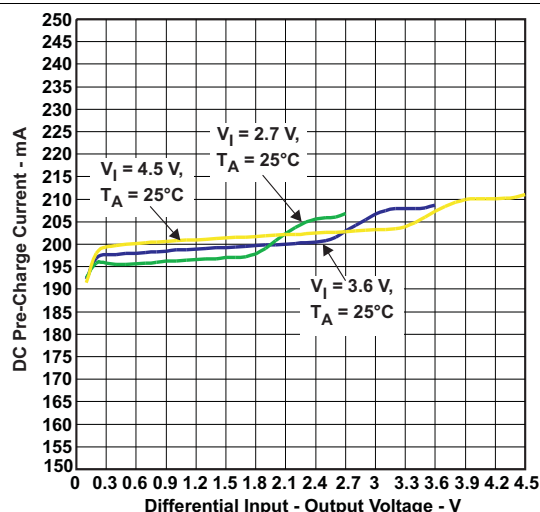
Figure 20. DC Pre-Charge Current vs Differential Input-Output Voltage
