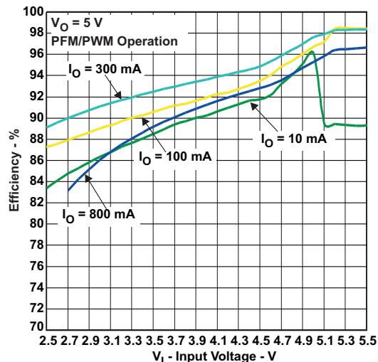
Figure 4. Efficiency vs Input Voltage
