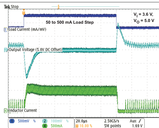
Figure 32. Load Transient Response in PFM/PWM Operation
