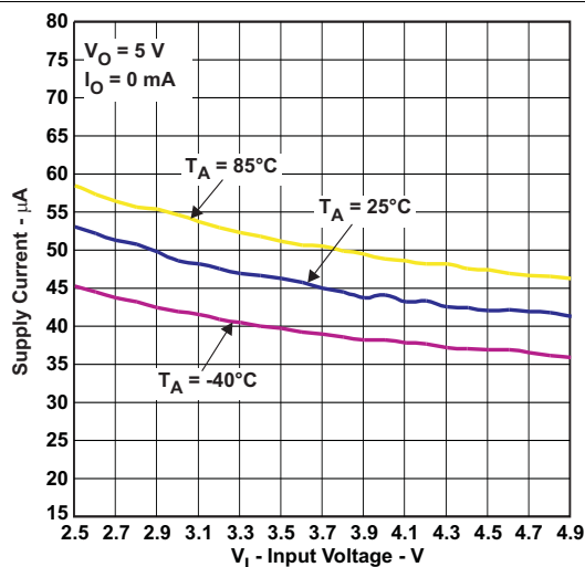
Figure 18. Supply Current vs Input Voltage
