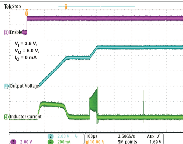
Figure 36. Start-Up
