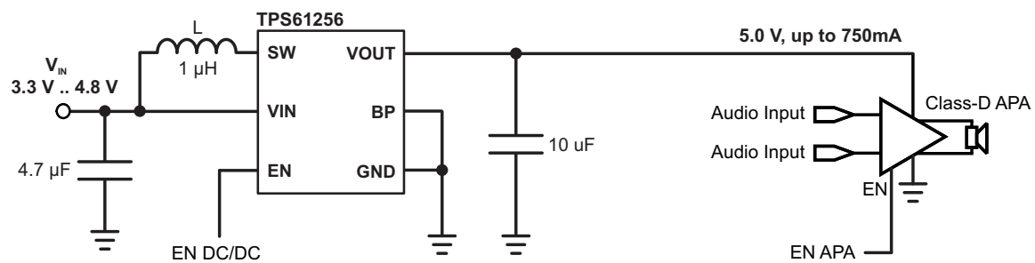
Figure 41. "Boosted" Audio Power Supply
