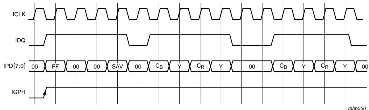
Fig 34. Output timing I port for serial 8-bit data at start of a line (ICODE = 1)
