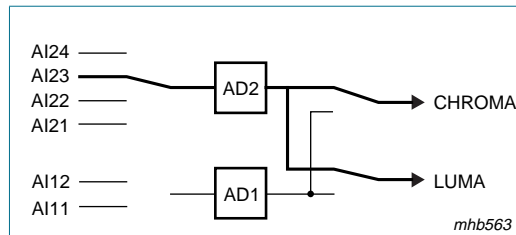
Fig 46. Mode 4 CVBS (automatic gain)
