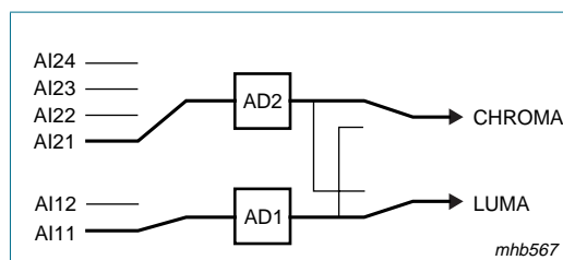
Fig 48. Mode 6 Y+ C (gain channel 2 adjusted via GAI2)
