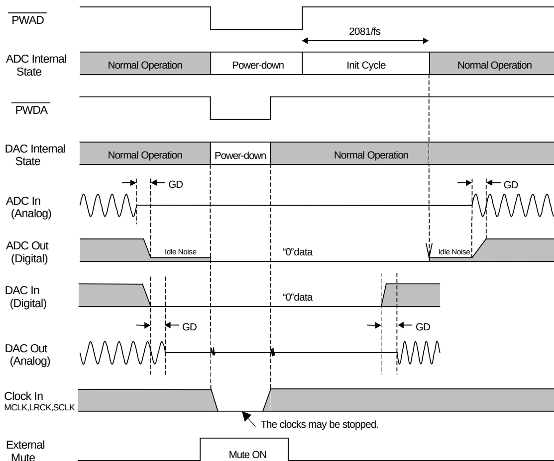
Figure 2. Power-up Sequence
