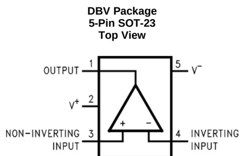
Pin Functions
