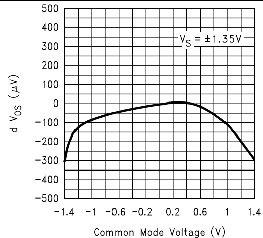
Figure 6. dV_{OS} vs Common Mode Voltage
