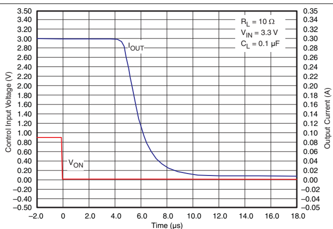
Figure 23. t_{OFF} Response
