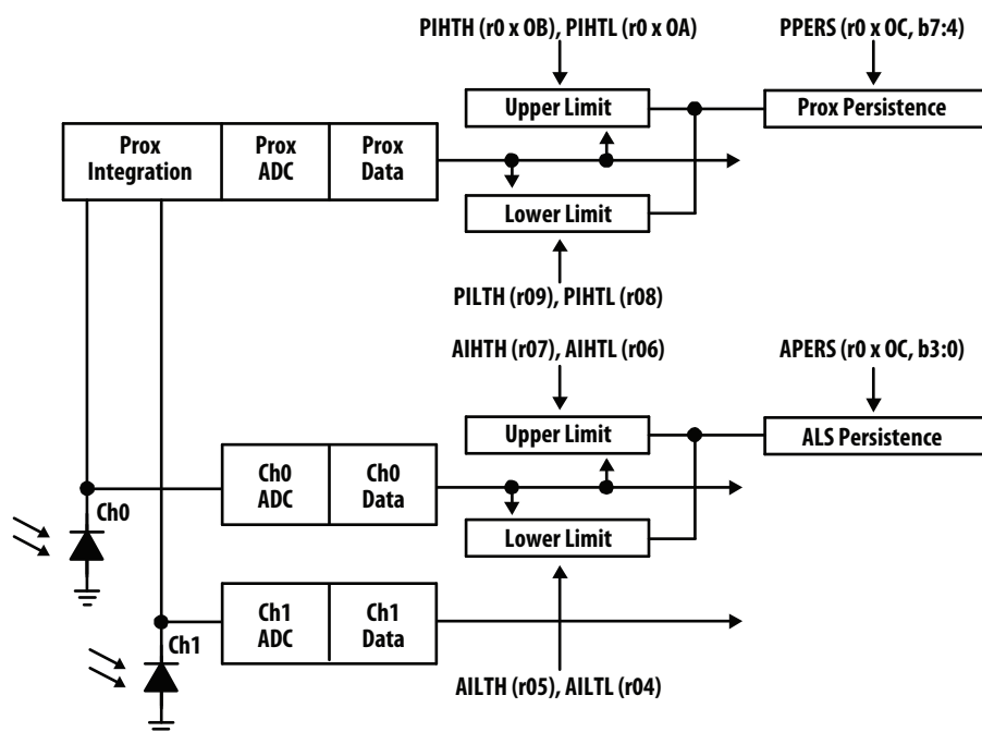
Figure 12. Programmable Interrupt
