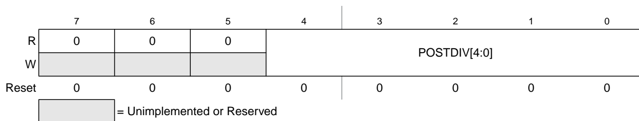
Figure 7-5. S12XECRG Post Divider Register (POSTDIV)
