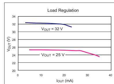
Figure 18. Load Regulation for LCD TV, Plasma TV Bias, FED Display, Varactor Diode Bias; V_{SUPPLY} = 5 V (circuit also shown in figure 3)
