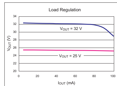
Figure 19. Load Regulation for LCD TV, Plasma TV Bias, FED Display, Varactor Diode Bias; V_{SUPPLY} = 12 V (circuit also shown in figure 4). The A8483 can operate with a V_{SUPPLY} from 0.9 to 18 V with a separate bias supply to operate the A8483 in the normal V_{IN} range. The bias voltage can be supplied by an external power supply, such as 3.3 or 5 V, or by using a suitable Zener diode, V_Z , for V_{SUPPLY} > 10 V.
