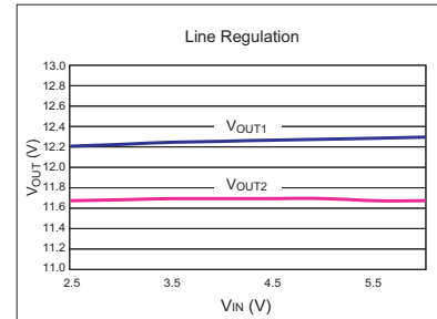
Figure 17. Line Regulation Performance for Small LCD Bias Supply, I_{OUT1} = I_{OUT2} = 7.5 mA (circuit also shown in figure 2)
