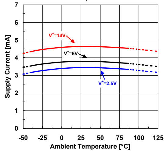
Supply Current vs. Temperature G_V=0\text{dB}
