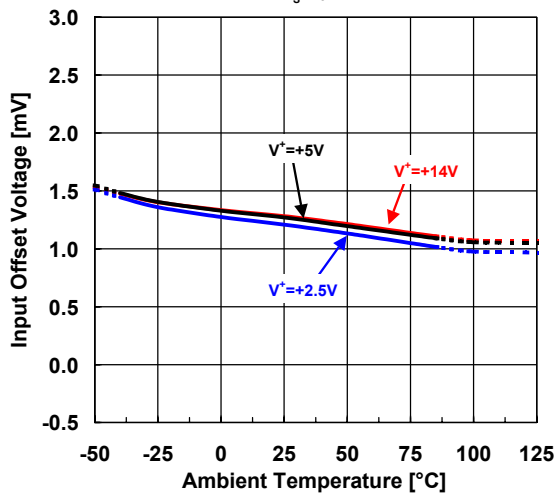
Input Offset Voltage vs. Temperature R_S=10\text{k}\Omega
