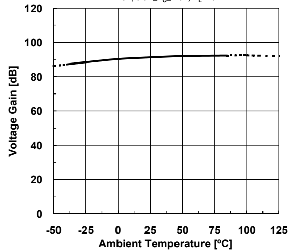
Large Signal Voltage Gain vs. Temperature V'=5\text{V}, 0.5\text{V} \leq V_O \leq 4.5\text{V}, R_L=10\text{k}\Omega
