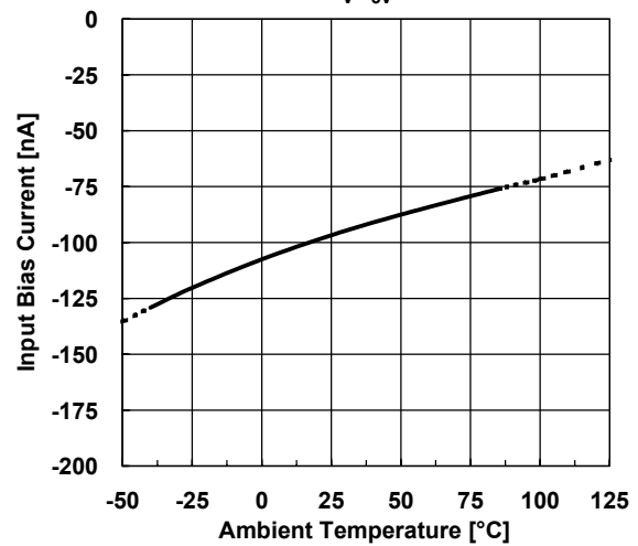
Input Bias Current vs. Temperature V'=5\text{V}
