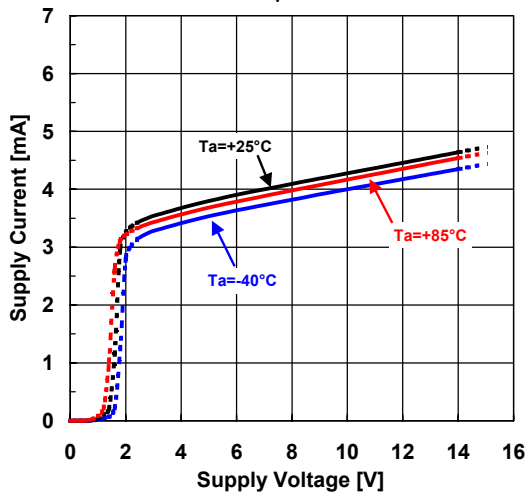
Supply Current vs. Supply Voltage G_V=0\text{dB}
