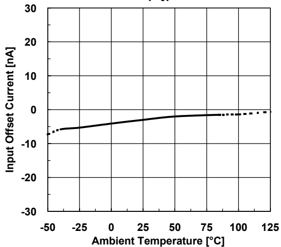
Input Offset Current vs. Temperature V'=5\text{V}
