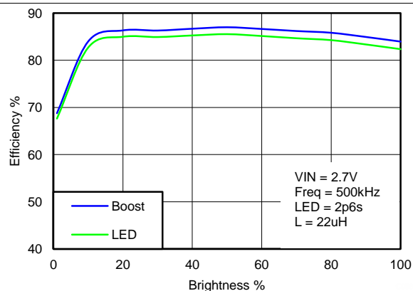
Figure 2. Boost and LED Efficiency
