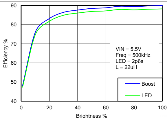
Figure 3. Boost and LED Efficiency
