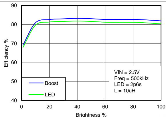
Figure 4. Boost And LED Efficiency
