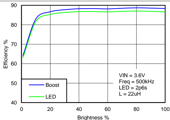
Figure 1. Boost and LED Efficiency
