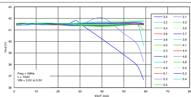
Figure 89. Maximum Boost Output Power vs V_{IN}
