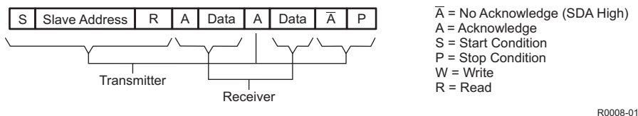
Figure 56. I²C Read Cycle
