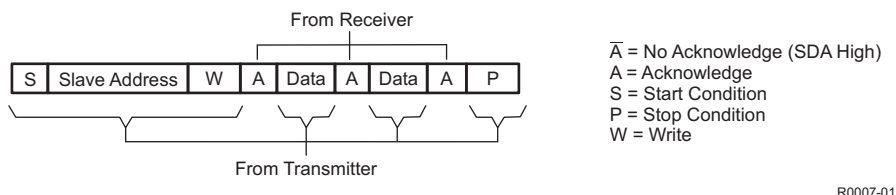
Figure 54. I²C Write Cycle
