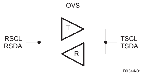
Figure 40. I 2 C Drivers in the TMD5261B (R Side Is the HDMI Source Side, T Side Is the HDMI Sink Side)
