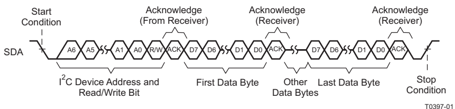
Figure 55. Multiple-Byte Write Transfer
