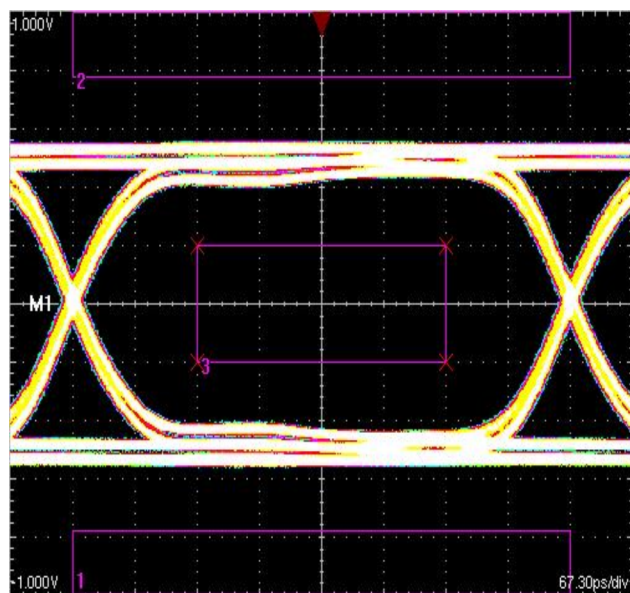
Figure 37. TMD5 Data Rate of 1856.25 Mbps
