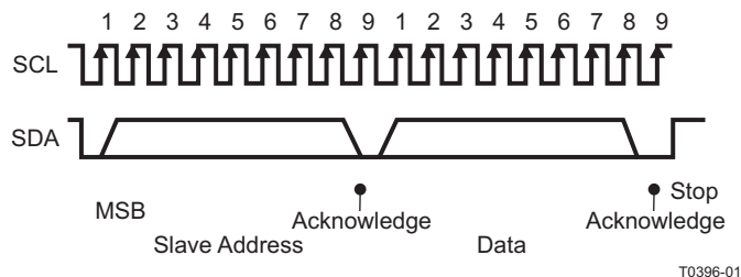
Figure 53. I²C Address, Data Cycle(s), and Stop
