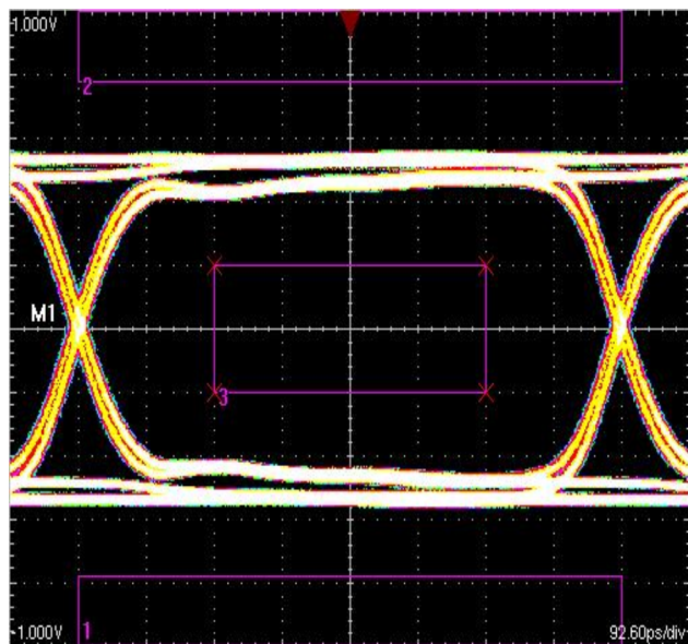
Figure 35. TMD5 Data Rate of 1350 Mbps
