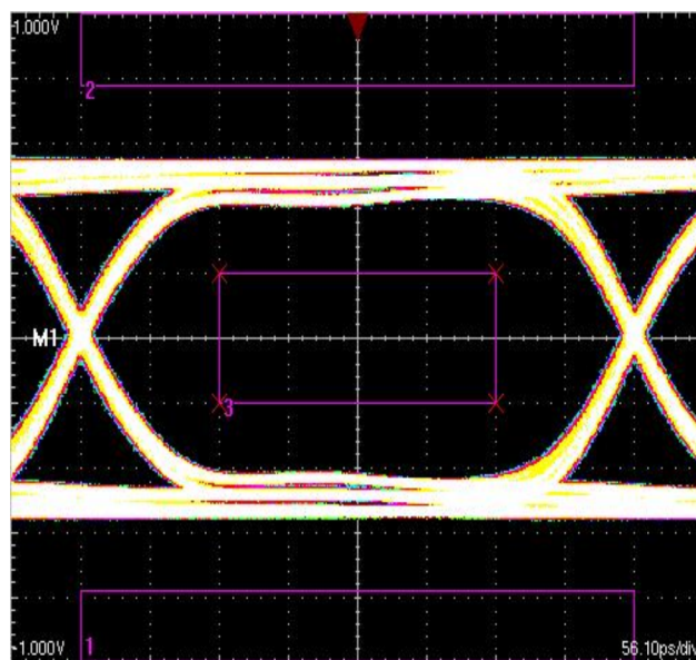
Figure 38. TMD5 Data Rate of 2227.5 Mbps
