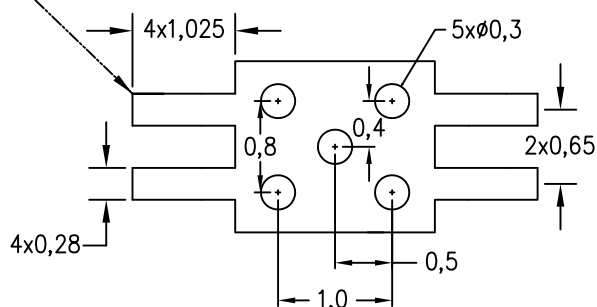
Example Solder Mask Opening (Note F) Pad Geometry (Note C)
