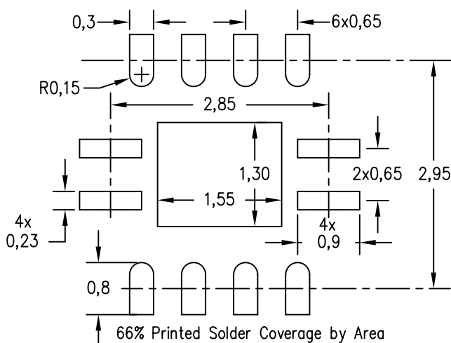
Example Stencil Design 0,125mm Stencil Thickness (Note E)
