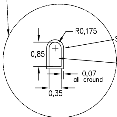
Example Non Solder Mask Defined Pad
