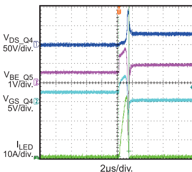
The Moment LED+ Short to LED- during Normal Operation
