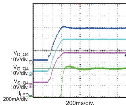
The Moment LED+ Short to LED- during Normal Operation
