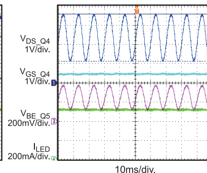
Steady State with Dimmer
