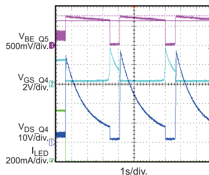
LED+ Short to LED- during Normal Operation
