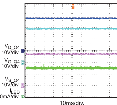
LED+ Short to LED- during Normal Operation
