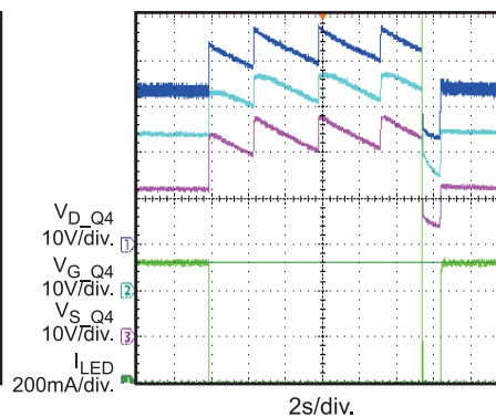
Output Open at Normal Operation then Recovery
