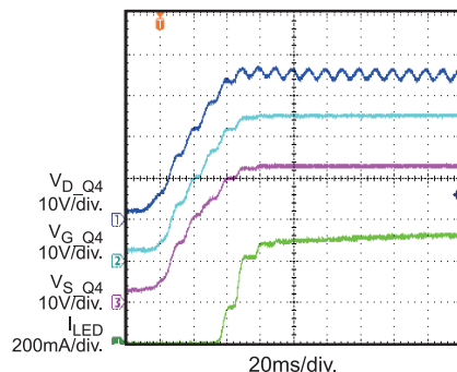
Start-up with Dimmer
