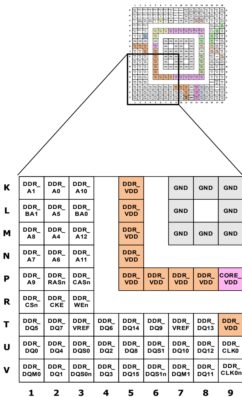
Figure 6-39. Bottom-Left Quadrant
