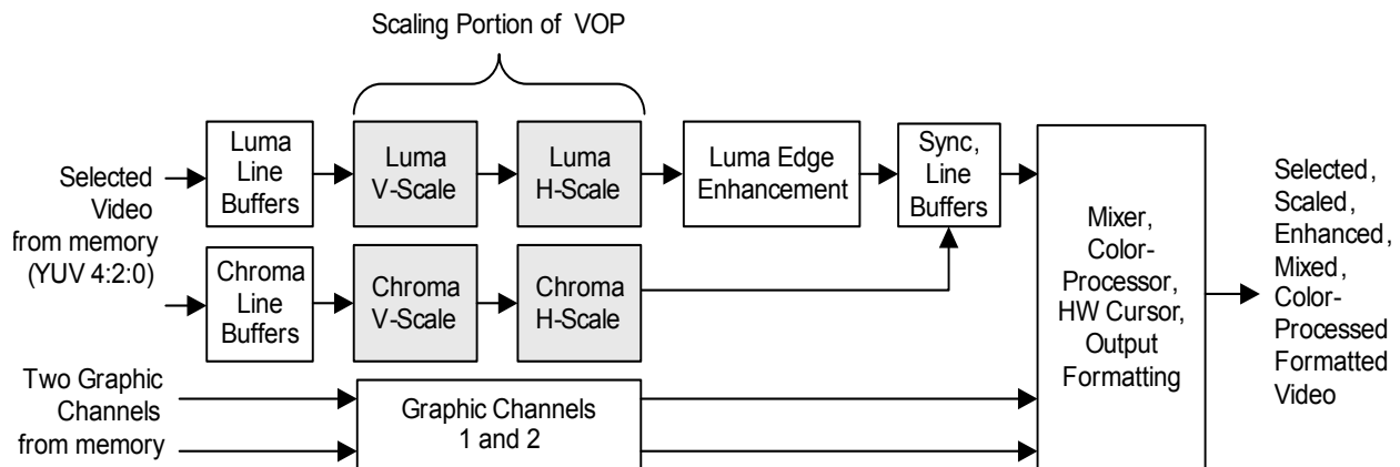
Figure 3-6. Video Output Processing Data Flow
