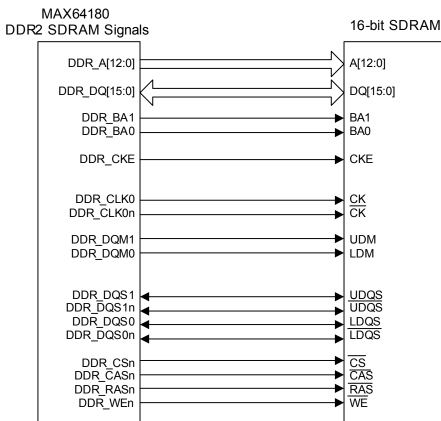
Figure 3-9. DDR2 SDRAM Connections for 512Mb 16-Bit
