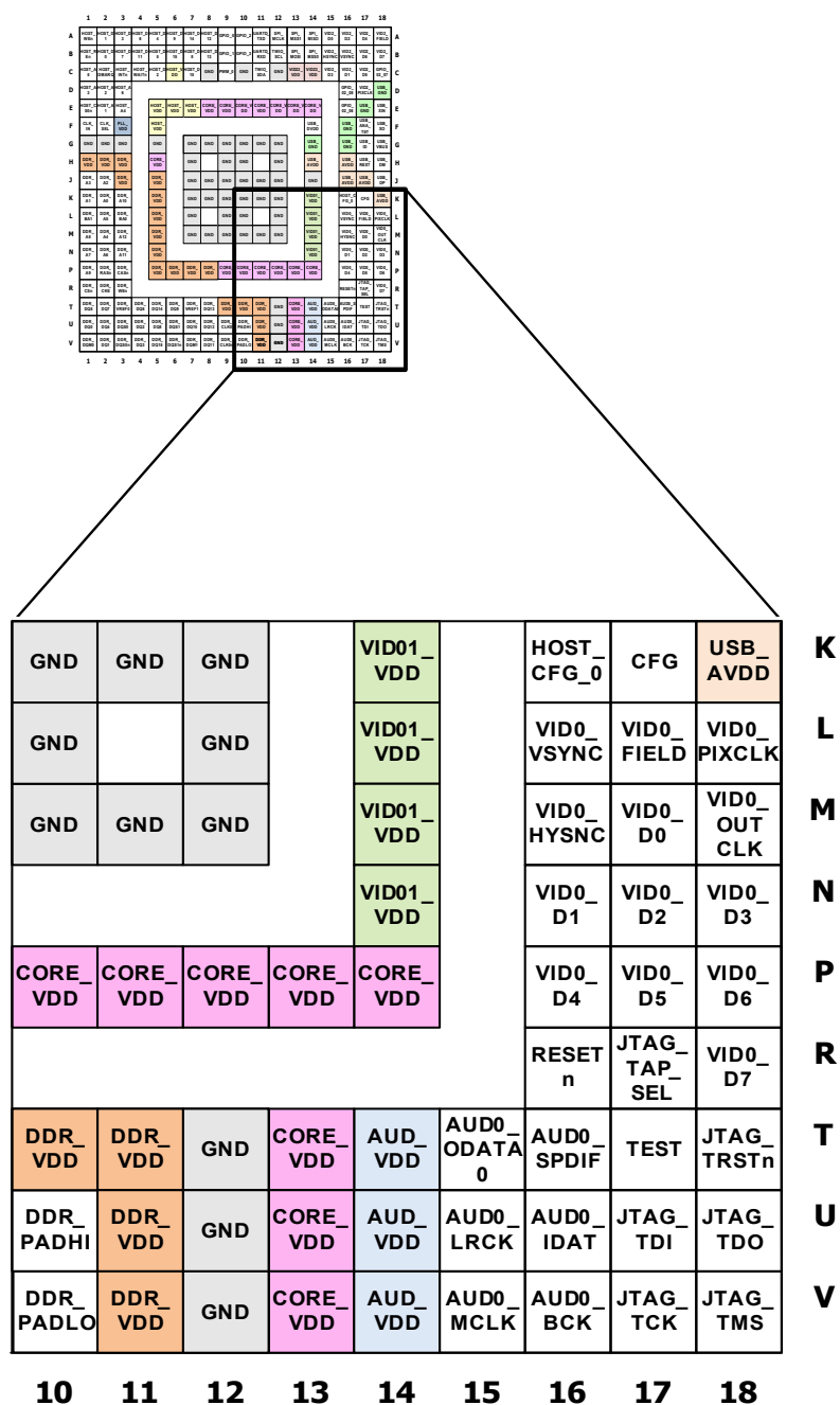
Figure 6-40. Bottom-Right Quadrant
