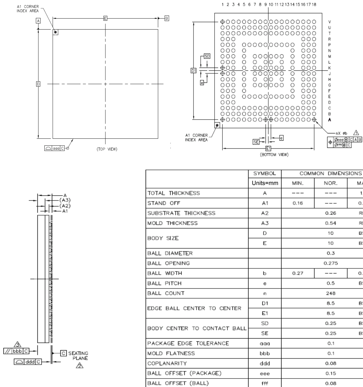
Figure 7-41. MAX64180 248-Pin CTBGA Package Physical Drawing
