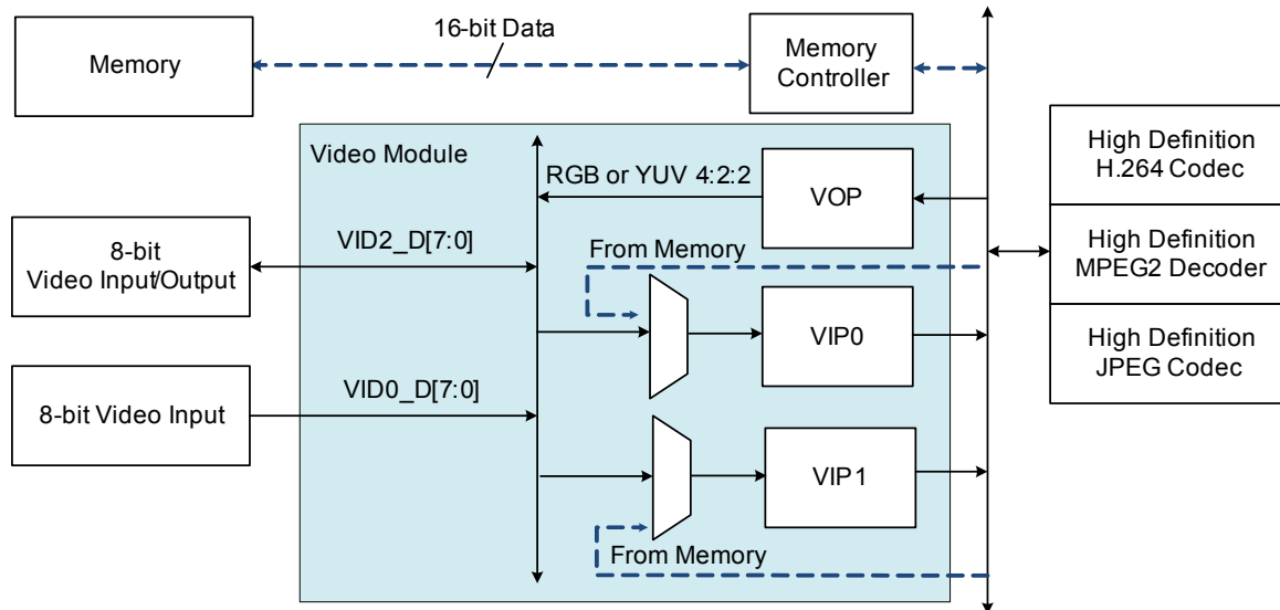
Figure 3-3. Video Subsystem
