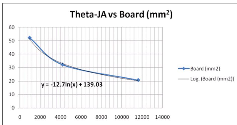
Figure 7-42. Thermal Resistance
