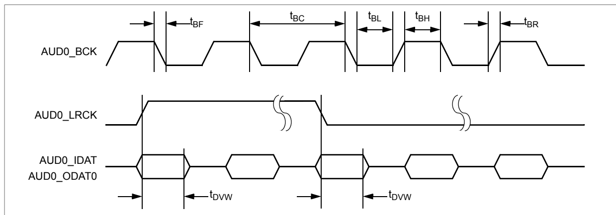
Figure 5-27. Audio Interface Timing
