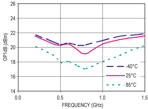
Figure 39. OP1dB vs Frequency ( V_d = 5V , I_{ds} = 15mA )
