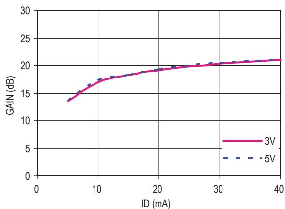
Figure 51. Gain vs Id( 100 MHz )
