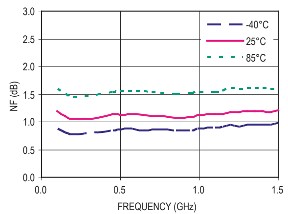
Figure 9. NF vs Frequency ( V_d = 3V , I_{ds} = 5mA )
