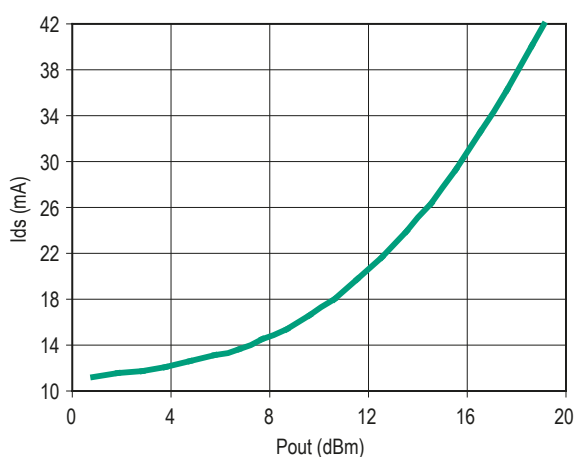
Figure 54. Ids vs Pout (Vd = 5V)
