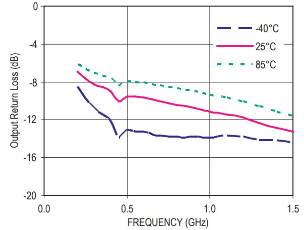
Figure 11. Output Return Loss vs Frequency ( V_d = 3V , I_{ds} = 5mA )
