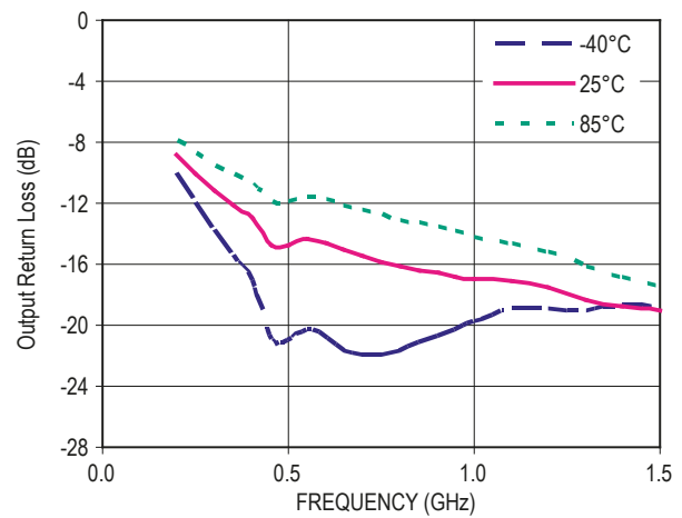
Figure 38. Output Return Loss vs Frequency ( V_d = 5V , I_{ds} = 10mA )
