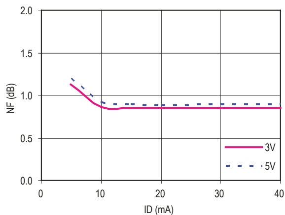
Figure 52. NF vs Id ( 100 MHz )
