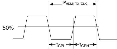
Figure 59. TMDS Clock Signal Definitions
