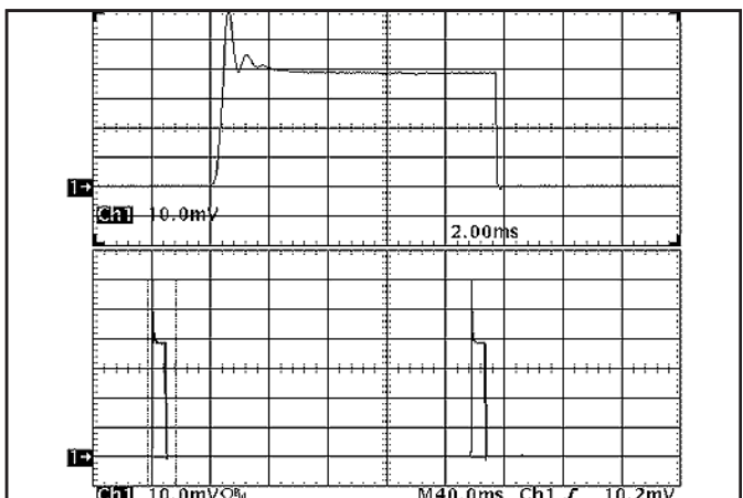
Figure 18: Load current (5A/div) as a function of time when the converter attempts to turn on into a 1 m \Omega short circuit. Top trace (2ms/div) is an expansion of the on-time portion of the bottom trace.
