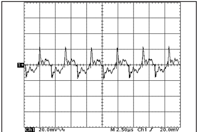
Figure 16: Output voltage ripple at nominal input voltage and rated load current (20 mV/div). Load capacitance: 1 \mu F ceramic capacitor and 15 \mu F tantalum capacitor. Bandwidth: 20 MHz. See Figure 13.
