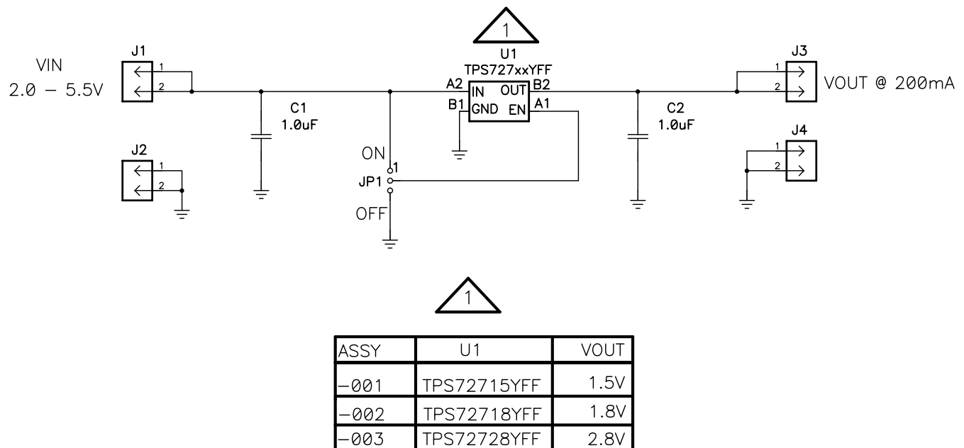
Figure 25. TPS727xxYFFEVM-407 Schematic
