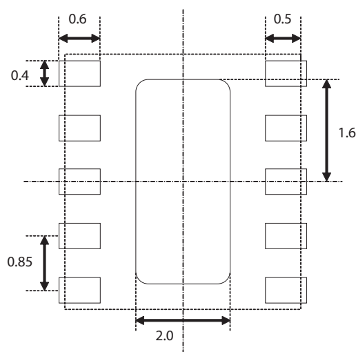
Figure 20. Solder Paste Stencil Aperture
