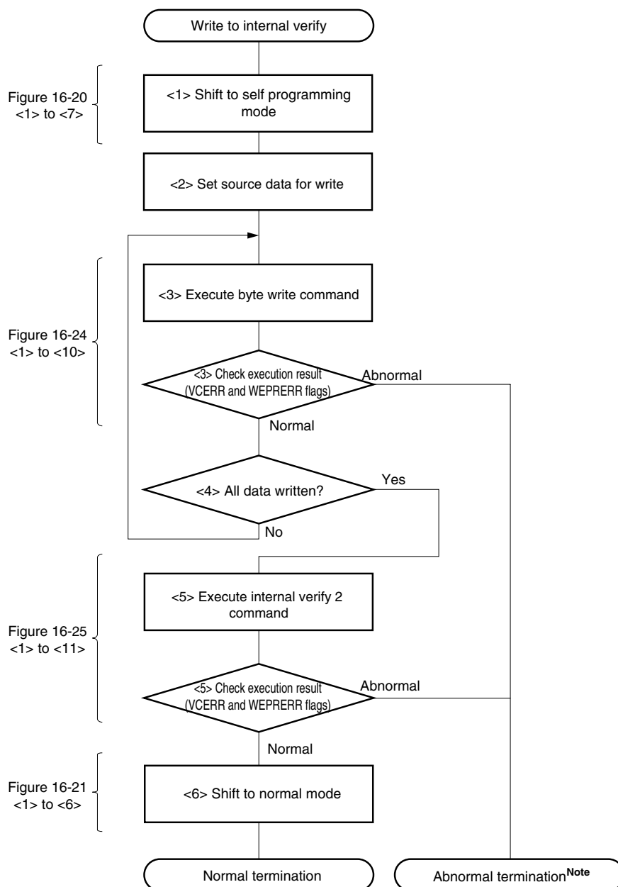
Figure 16-28. Example of Operation When Command Execution Time Should Be Minimized (from Write to Internal Verify)
