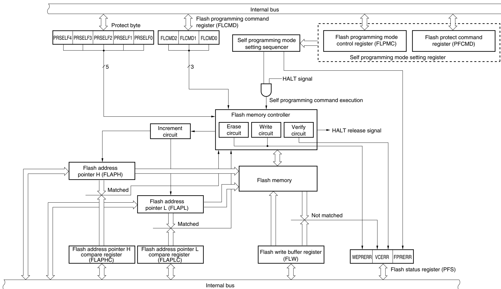
Figure 16-10. Block Diagram of Self Programming
