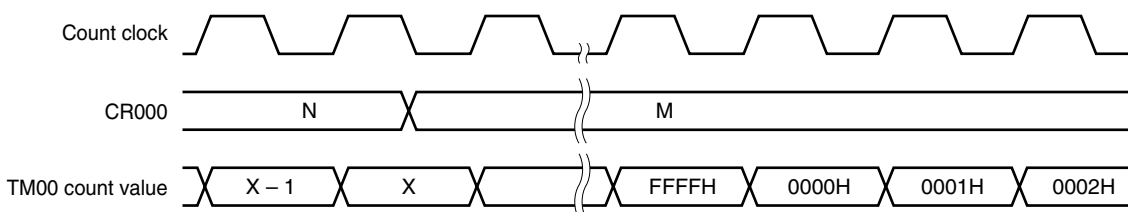
Figure 6-14. Timing After Change of Compare Register During Timer Count Operation (N → M: N > M)
