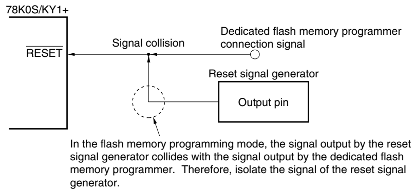
Figure 16-8. Signal Collision (RESET Pin)
