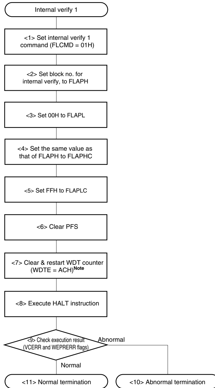
Figure 16-25. Example of Internal Verify 1 Operation in Self Programming Mode
