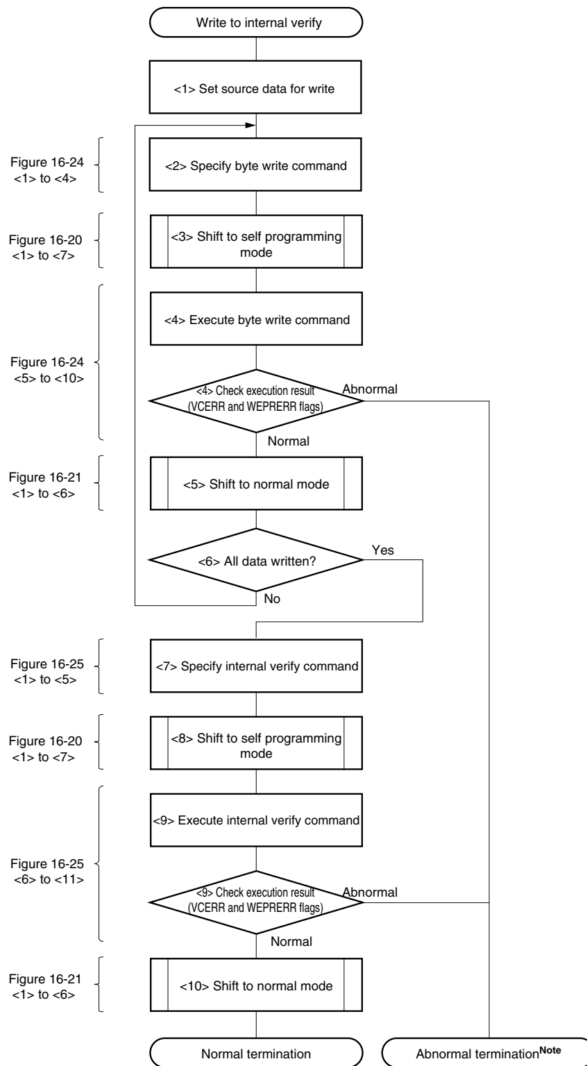
Figure 16-30. Example of Operation When Interrupt-Disabled Time Should Be Minimized (from Write to Internal Verify)
