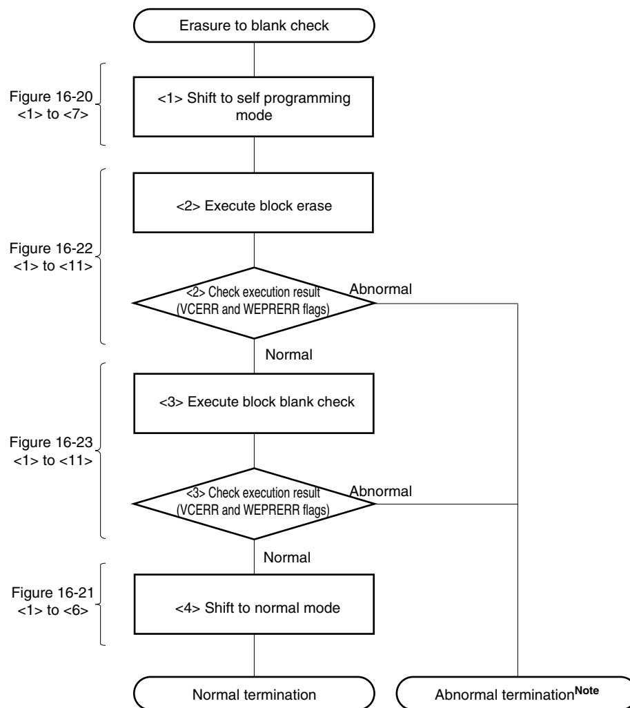
Figure 16-27. Example of Operation When Command Execution Time Should Be Minimized (from Erasure to Blank Check)
