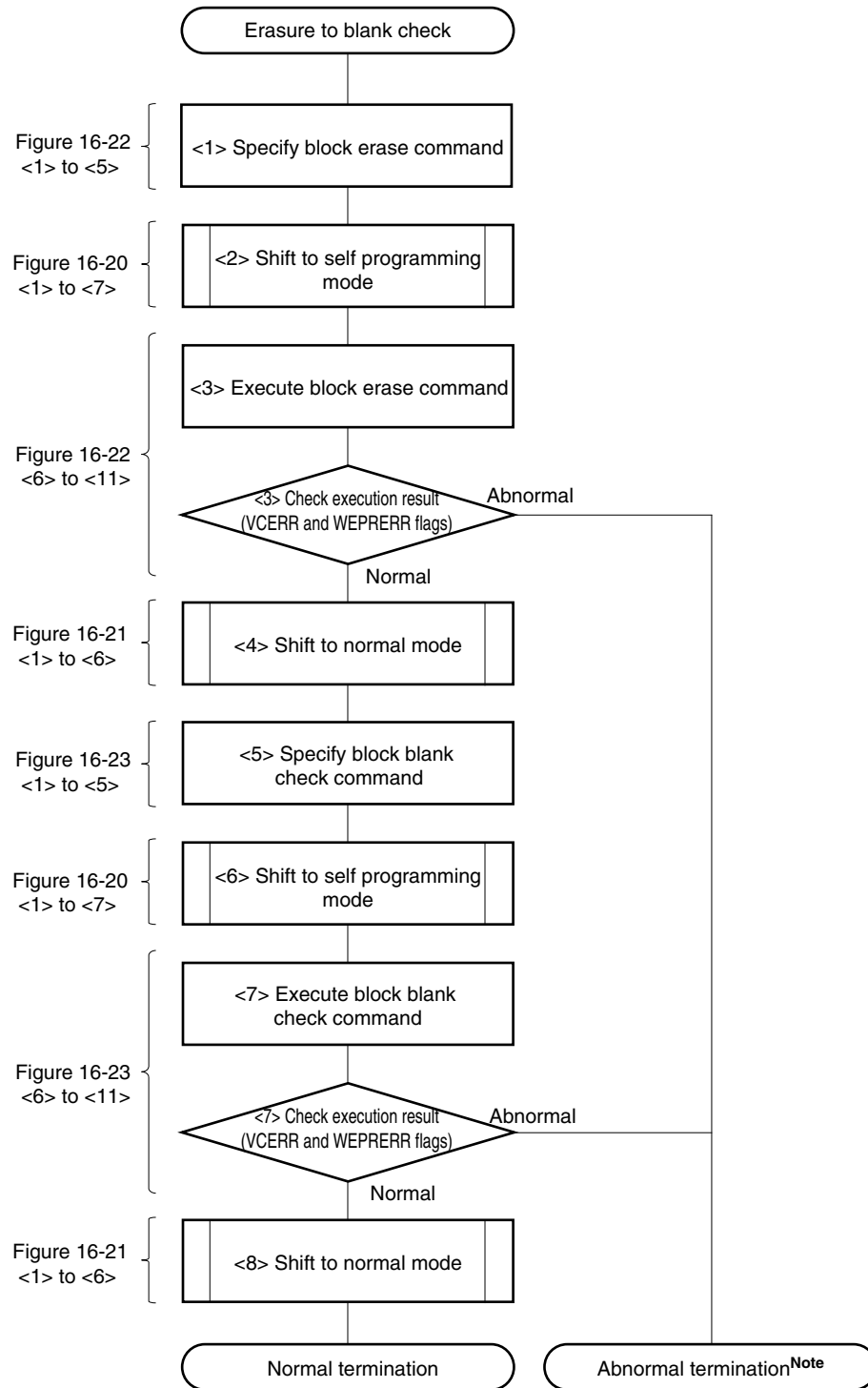
Figure 16-29. Example of Operation When Interrupt-Disabled Time Should Be Minimized (from Erasure to Blank Check)
