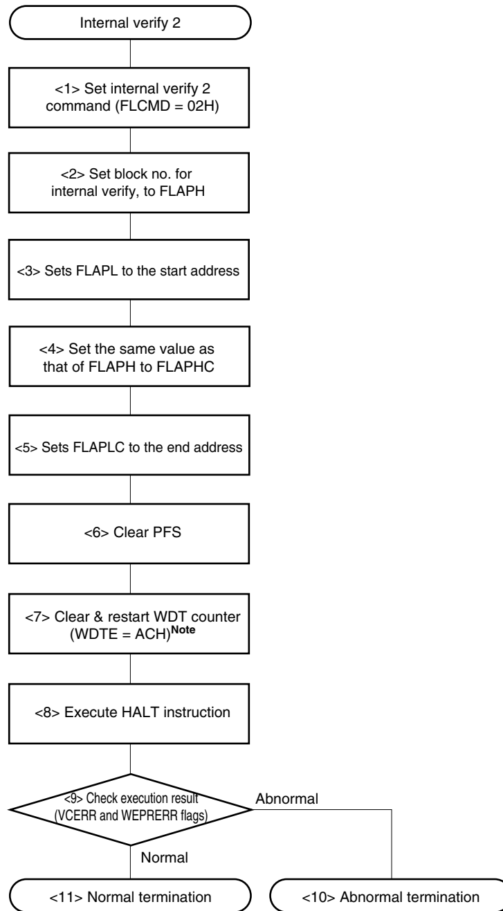
Figure 16-26. Example of Internal Verify 2 Operation in Self Programming Mode
