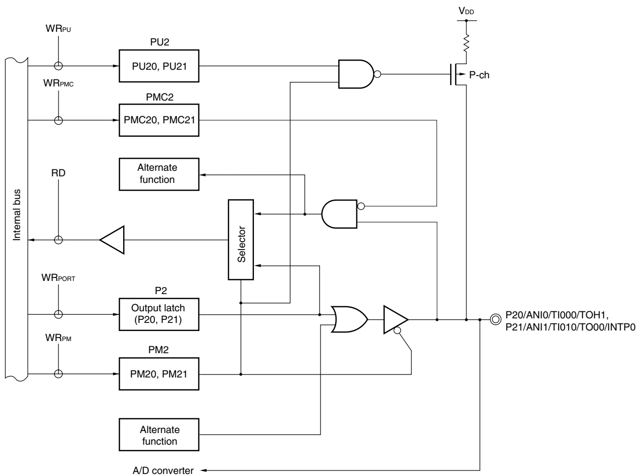
Figure 4-2. Block Diagram of P20 and P21
