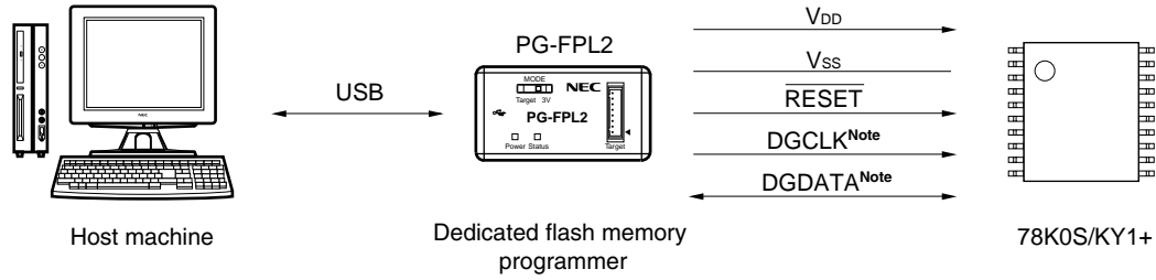
Figure 16-3. Environment for Writing Program to Flash Memory (PG-FPL2)
