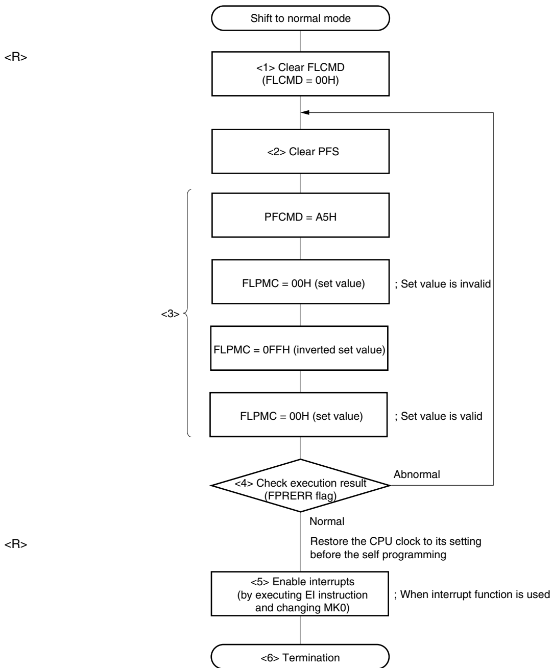
Figure 16-21. Example of Shifting to Normal Mode
