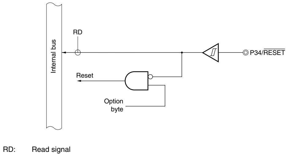
Figure 4-6. Block Diagram of P34
