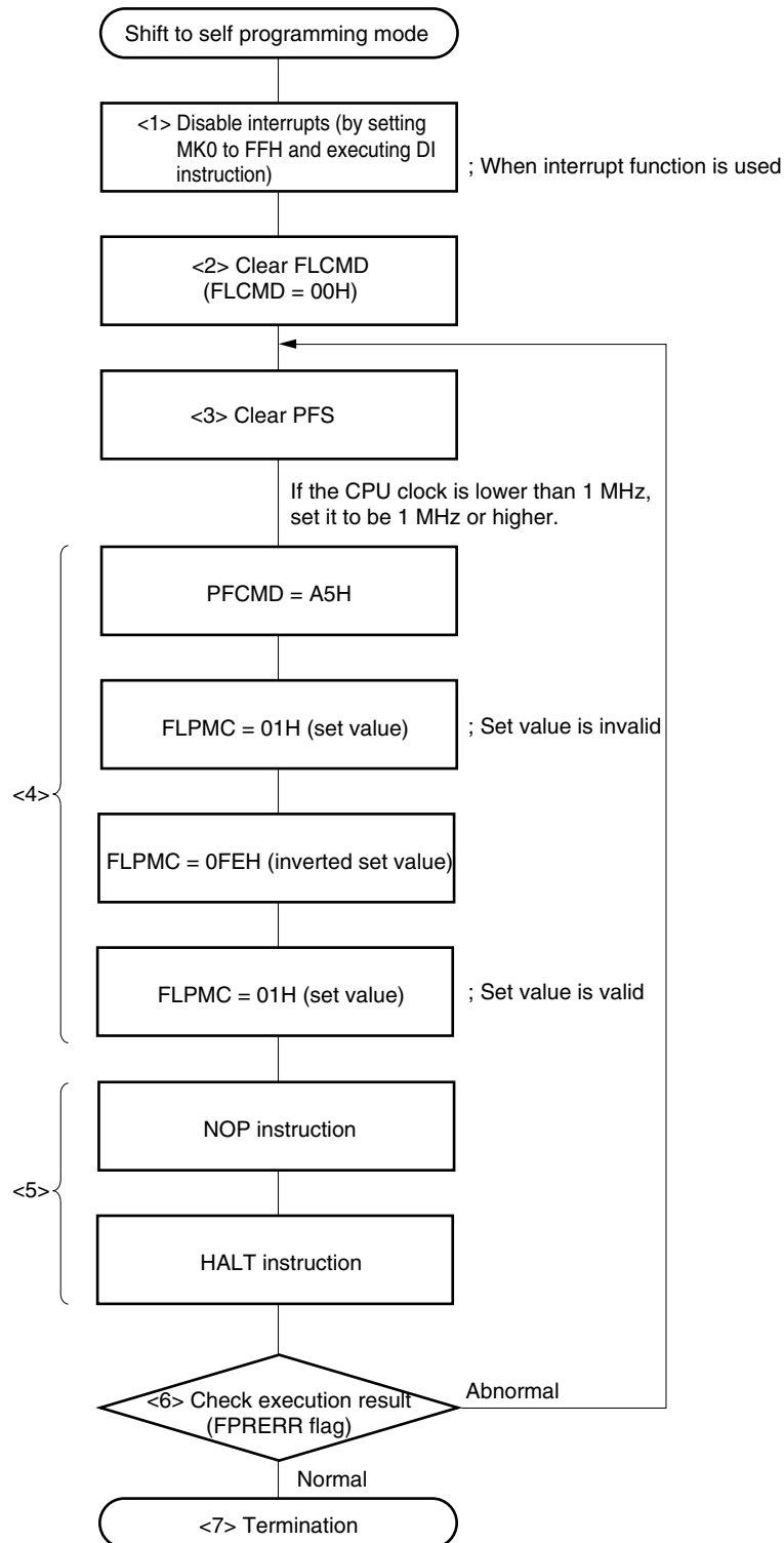
Figure 16-20. Example of Shifting to Self Programming Mode
