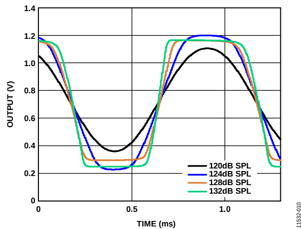
Figure 10. Clipping Characteristics
