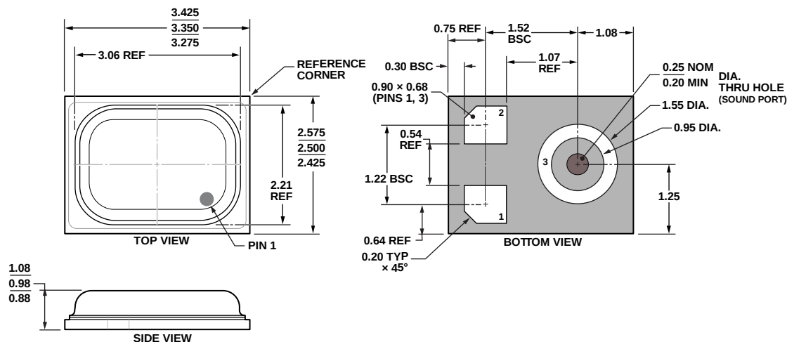
Figure 15. 3-Terminal Chip Array Small Outline No Lead Cavity [LGA_CAV] 3.35 mm × 2.5 mm Body (CE-3-5) Dimensions shown in millimeters
