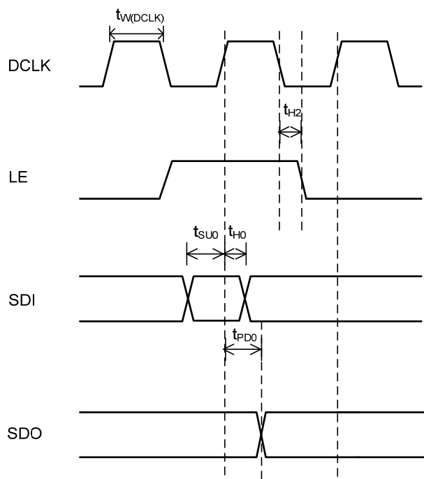
Timing Waveform for Global Latch
