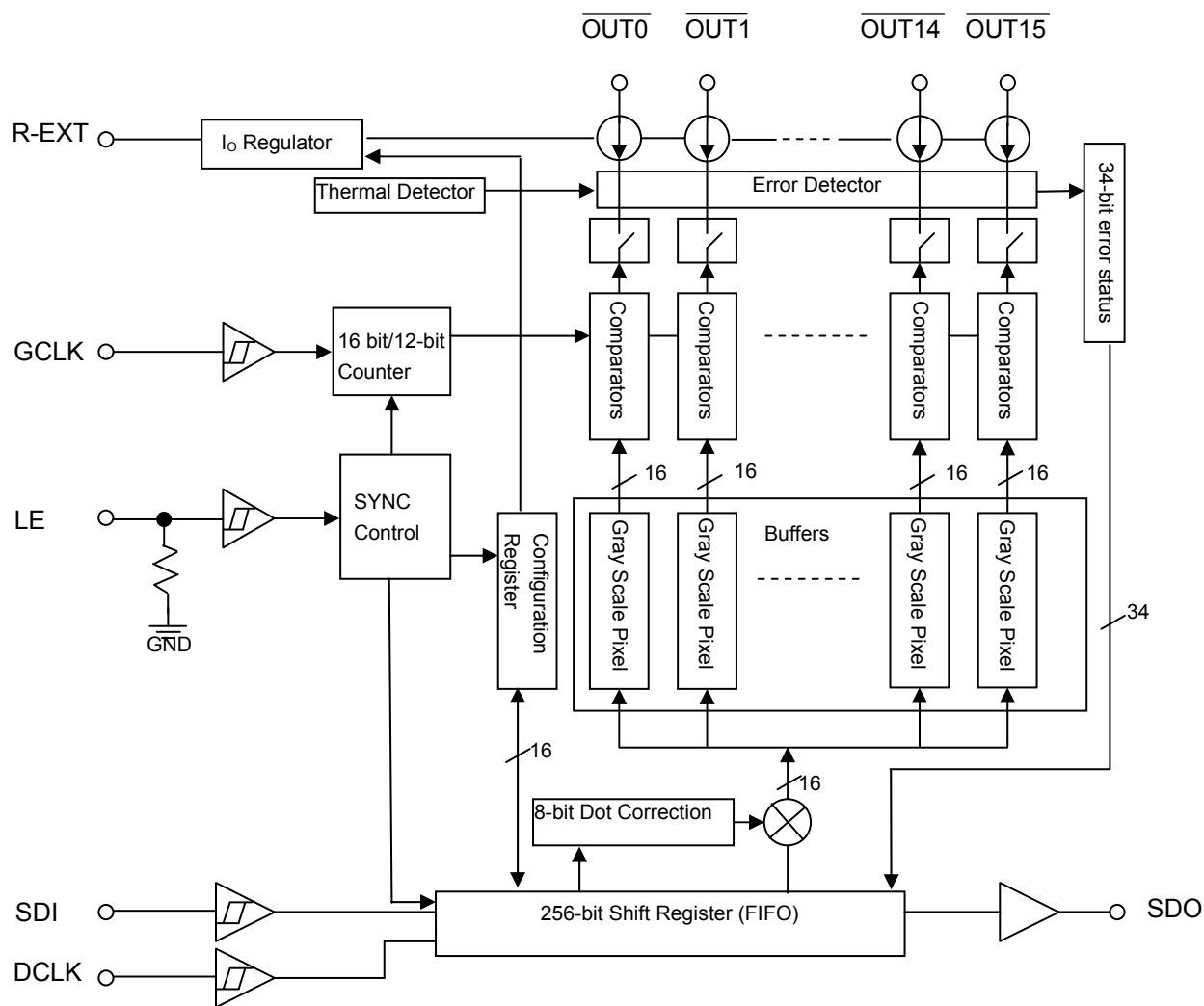
Block Diagram
