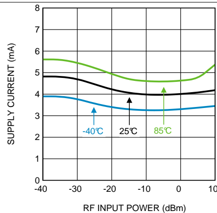
Figure 4. Supply Current vs. RF Input Power
