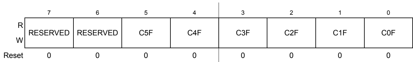
Figure 22-16. Main Timer Interrupt Flag 1 (TFLG1)
