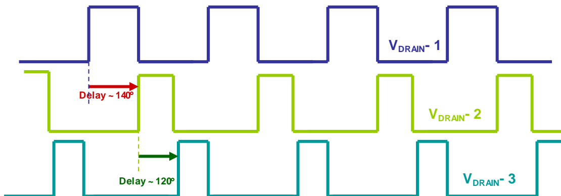
Figure 7: Example of a possible way to synchronize and use delays advantageously to minimize input ripple. R1 ~ 39k \Omega , R2 ~ 33k \Omega . (Refer to Figure 6 for R1 and R2.) R3 does not matter in this case.
